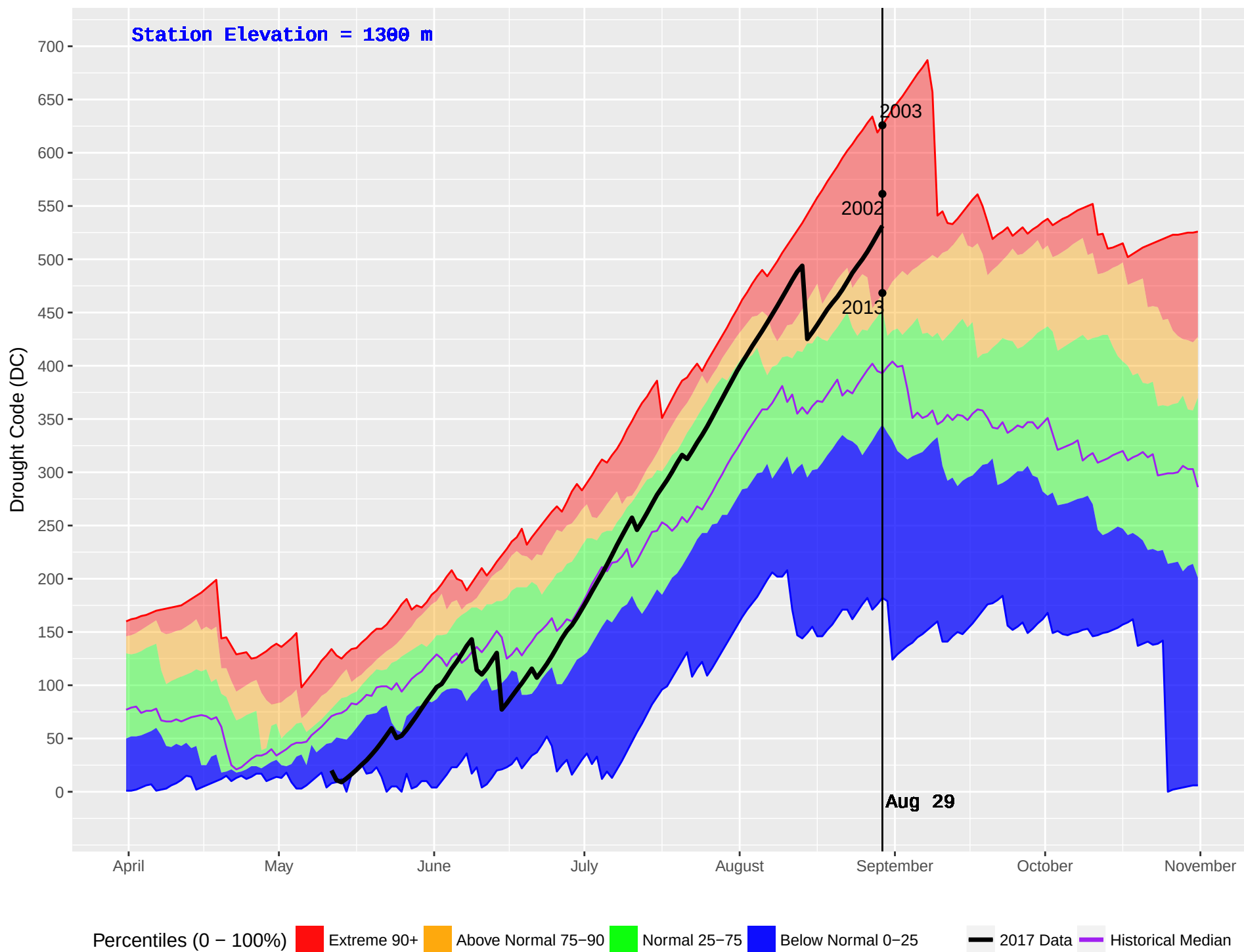
MARION (367) : Historical (1994–2016) and Current (2017) Noon Drought Code (DC)
