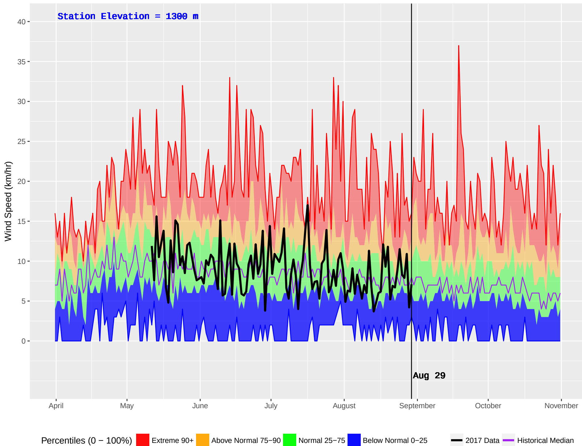
MARION (367) : Historical (1994–2016) and Current (2017) Noon Wind Speed
