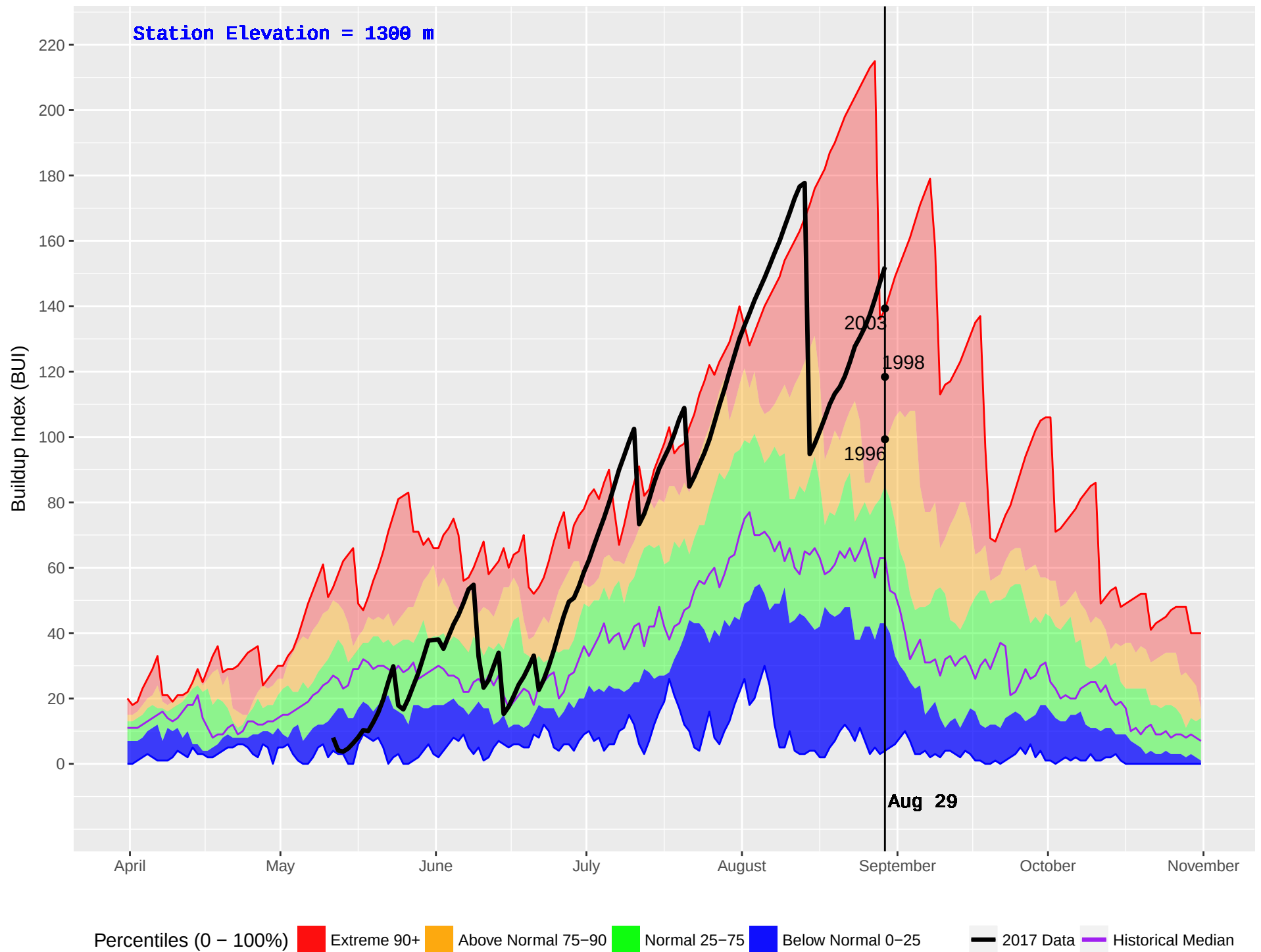
MARION (367) : Historical (1994–2016) and Current (2017) Noon Buildup Index (BUI)
