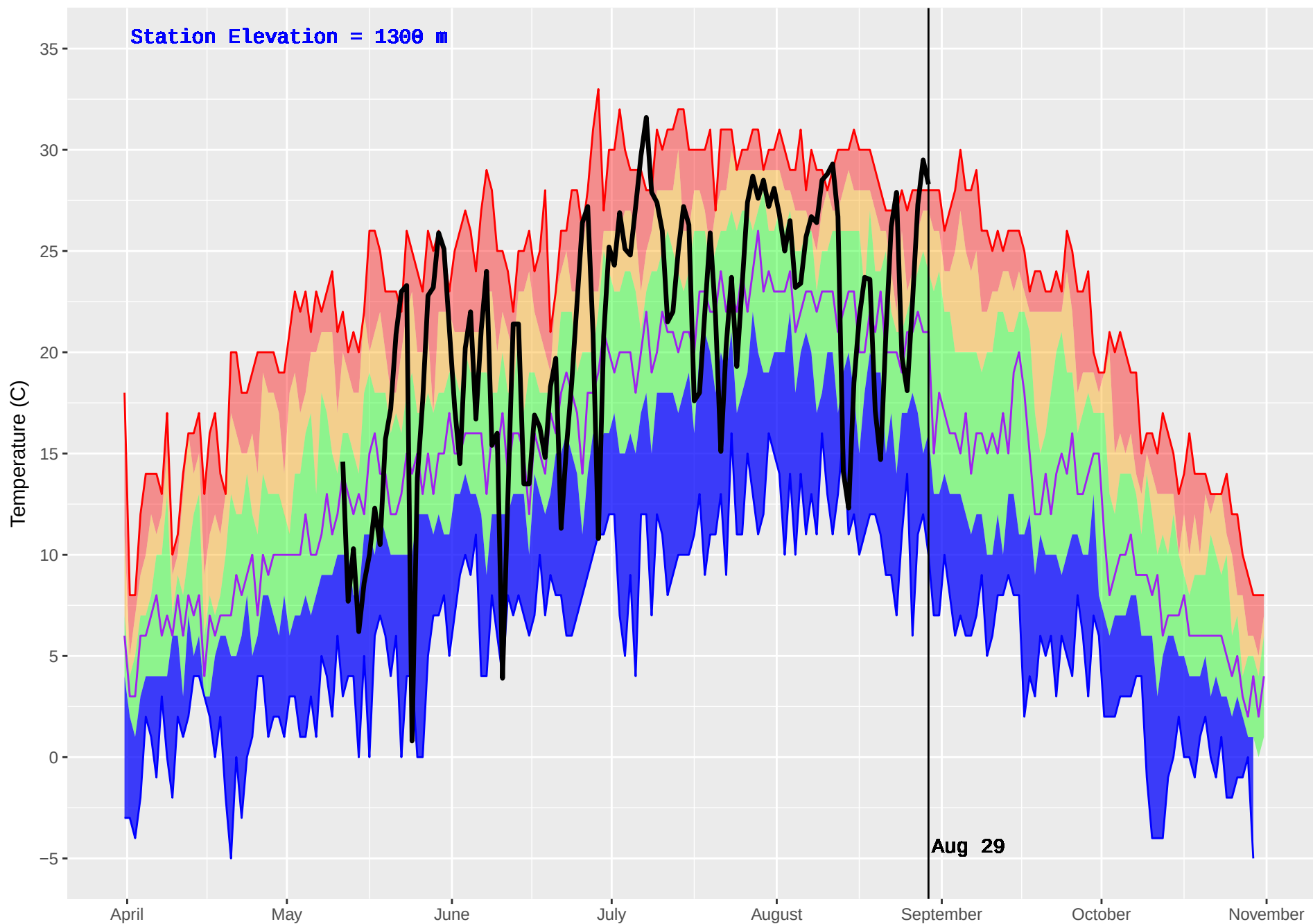
MARION (367) : Historical (1994–2016) and Current (2017) Noon Temperature
