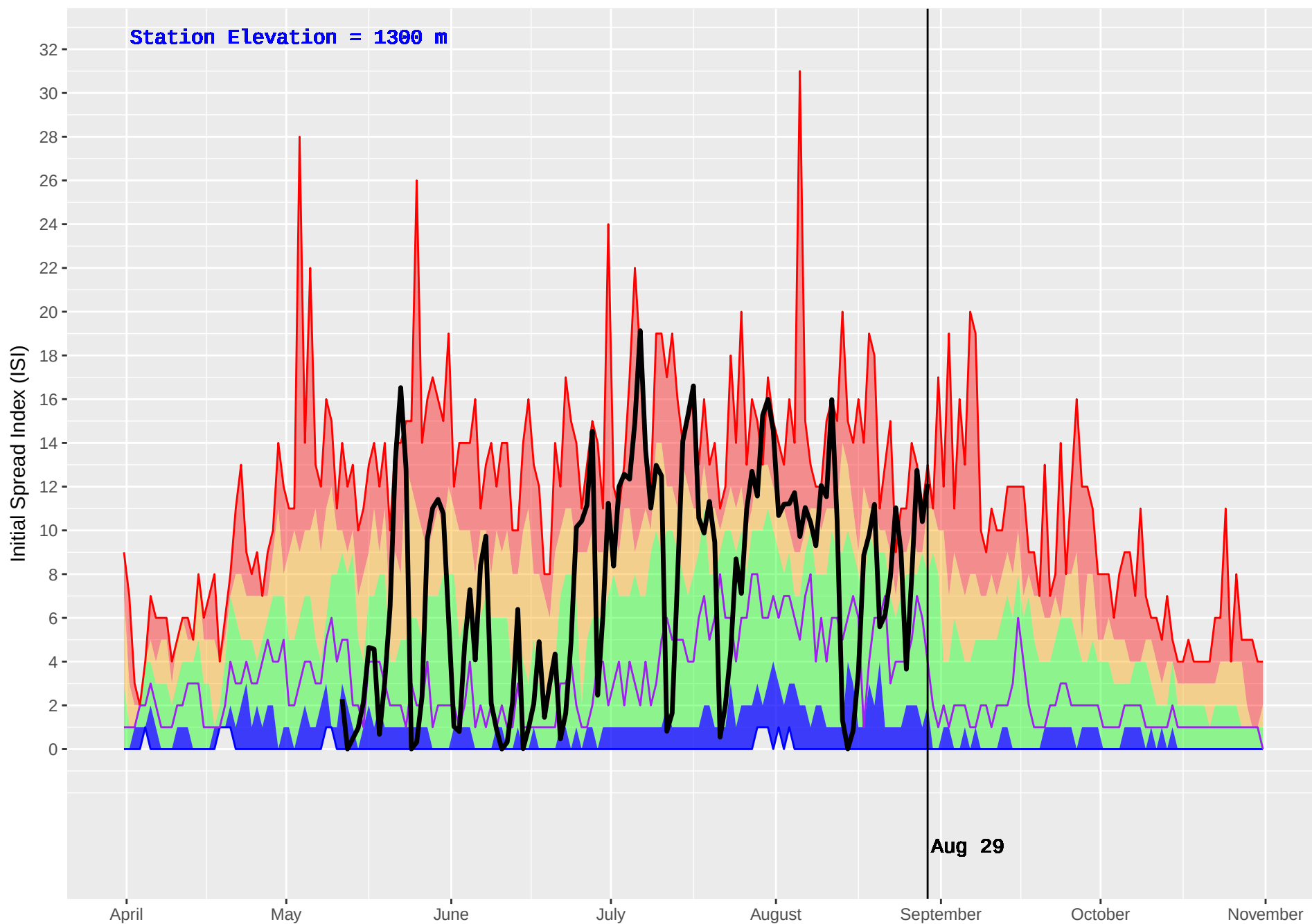
MARION (367) : Historical (1994–2016) and Current (2017) Noon Initial Spread Index (ISI)
