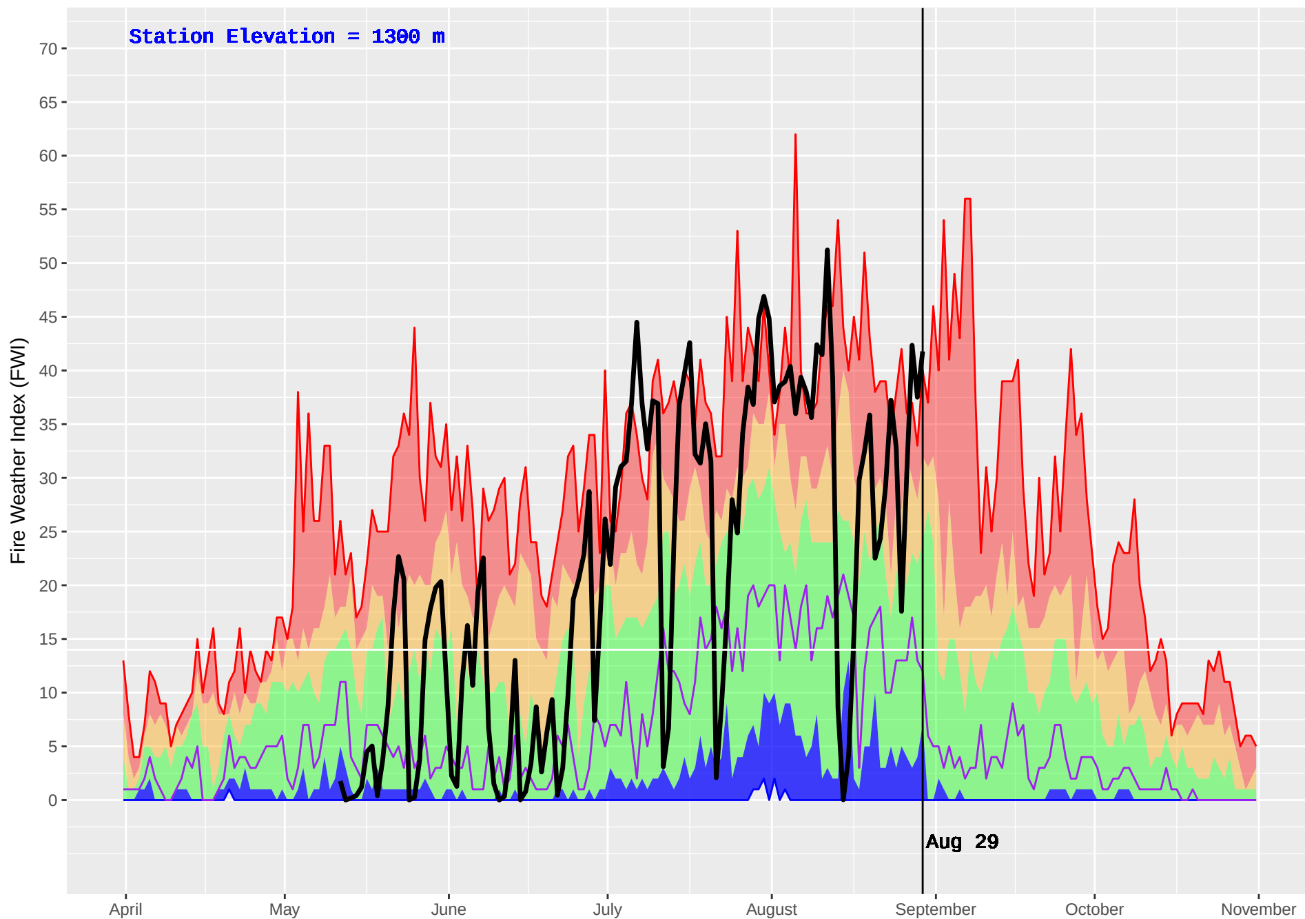
MARION (367) : Historical (1994–2016) and Current (2017) Noon Fire Weather Index (FWI)
