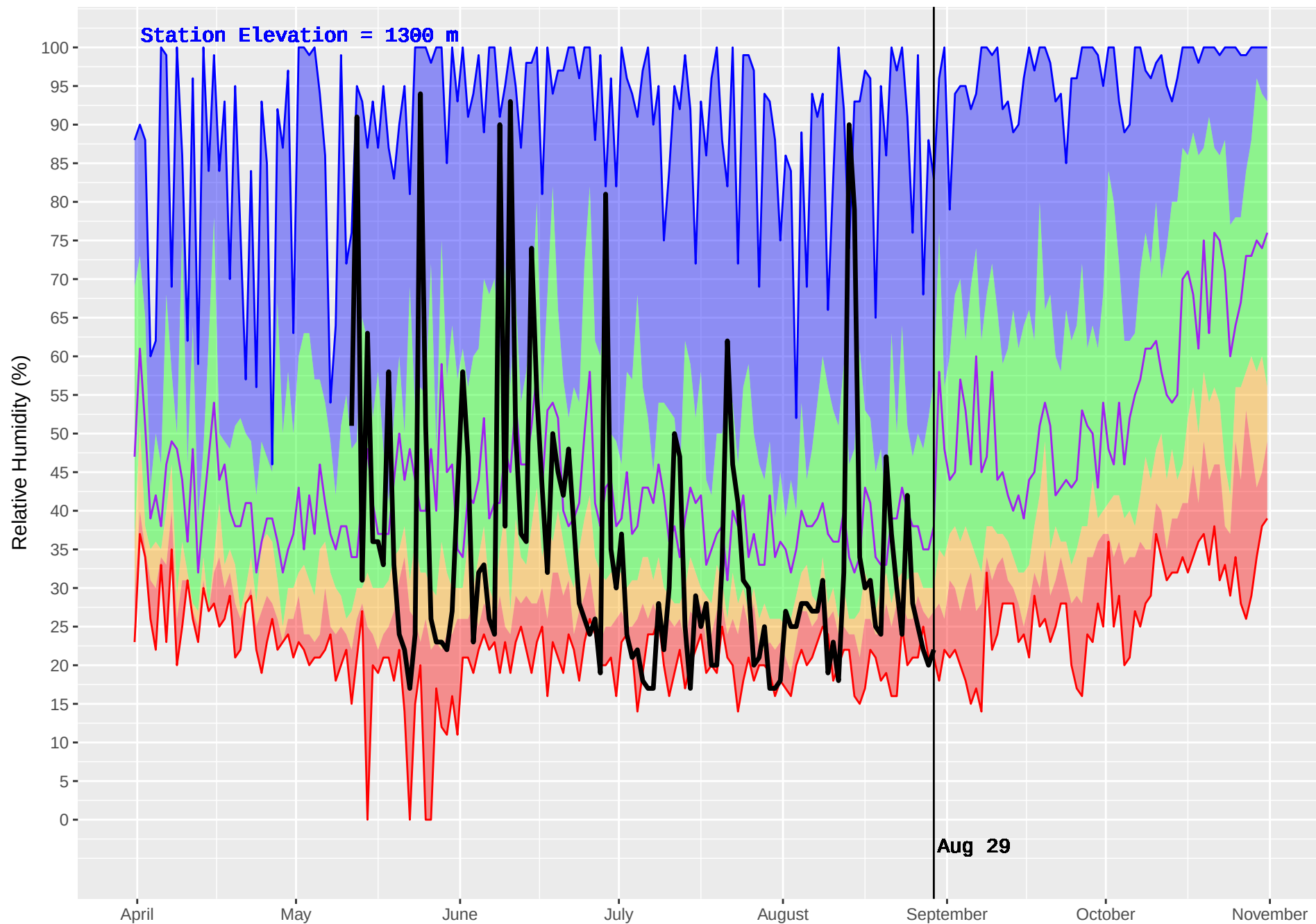
MARION (367) : Historical (1994–2016) and Current (2017) Noon Relative Humidity
